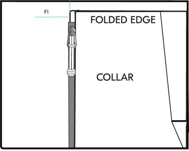
Option B, zipper stop 0,5 cm below CHINGUARD windfalp top end. Outside Right side
